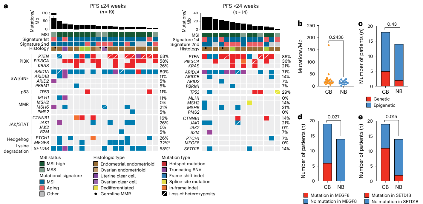
Fig. 4 | Somatic mutations in ovarian and endometrial cancers according to clinical benefit. a , TMB, MSIsensor score, mutational signatures and recurrent non-synonymous somatic mutations identified by whole-exome sequencing in endometrial cancers with clinical benefit (PFS \geq 24 weeks) and without clinical benefit (PFS < 24 weeks). Cases are represented by columns and genes by rows. Only pathogenic mutations are shown. MSI status, dominant mutational signature, histologic types and mutation types are color-coded according to the legend. Percentages in bold indicate statistically significantly different. * P < 0.05 , two-sided Fisher's exact test. First, dominant mutational signature;
