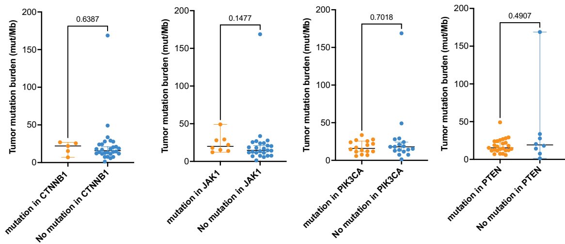
Extended Data Fig. 3 | Association of individual mutations with tumor mutational burden (TMB). Extended Data Fig. 3 Association of individual mutations with tumor mutational burden (TMB). Presence or absence of the individual mutations known to be associated with immune resistance in other
