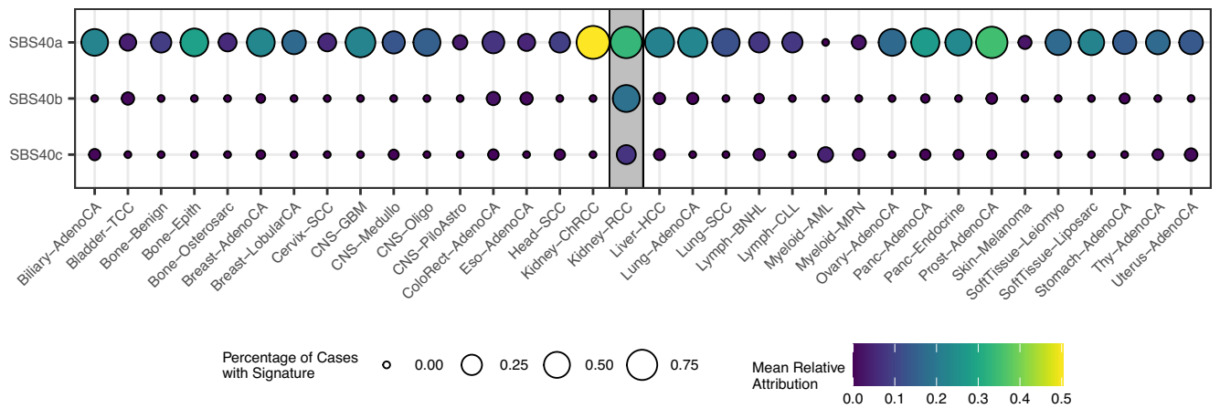
Extended Data Fig. 3 | Attribution of signatures SBS40a, SBS40b, and SBS40c in a pan-cancer cohort. Attribution of signatures SBS40a, SBS40b, and SBS40c in a pan-cancer cohort, showing a widespread distribution for SBS40a whilst SBS40b and SBS40c are only seen consistently in clear cell renal
