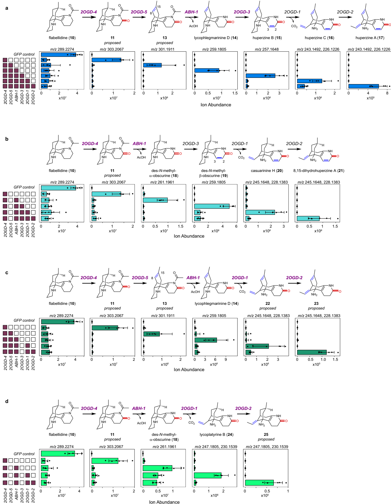
Extended Data Fig. 10 | Step-by-step biosynthesis of downstream Lycopodium alkaloids. a ) Generation of HupA (17). b ) Generation of 8,15-dihydro congeners. c ) Generation of 2,3-dihydro congeners. d ) Generation of 2,3,8,15-tetrahydro congeners. For all panels, filled in boxes to the left indicate presence of biosynthetic genes in our N. benthamiana transient expression system. Flabellidine (10) was co-infiltrated as a substrate in all experiments. Shown below each compound is the mean ion abundance for the indicated mass ions ( m/z ) for each compound. In all panels, n = 6 infiltrated leaves for
