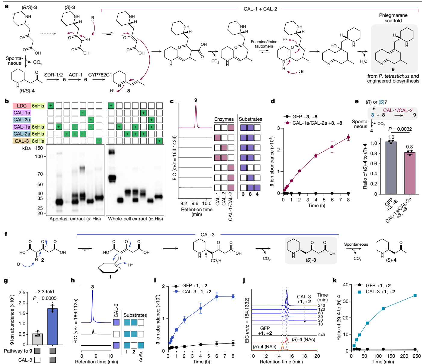
Fig. 3 | Neofunctionalized CAL enzymes in Lycopodium alkaloid biosynthesis. a , Proposed mechanism for biosynthesis of 9 by PtCAL-1a/PtCAL-2a. b , Representative western blot of 6xHis-tagged CALs expressed alone or co-expressed with untagged gene constructs in N. benthamiana . A 6xHis-tagged LcLDC construct was included as an intracellular control. This experiment was performed more than three times with similar results routinely observed. c , EICs for production of 9 ( m/z 164.1434) by apoplastic PtCAL-1a and PtCAL-2a (alone or co-expressed) with different substrate combinations. d , Time course of 9 production by apoplastic PtCAL-1a/PtCAL-2a compared to a GFP apoplastic control. n = 3 reactions per condition. e , Assessment of which 3 enantiomer is used as a substrate in the formation of 9 . Because 3 enantiomers could not be directly observed, chirality was inferred by measuring 4 enantiomers, which form through spontaneous decarboxylation of 3 .
