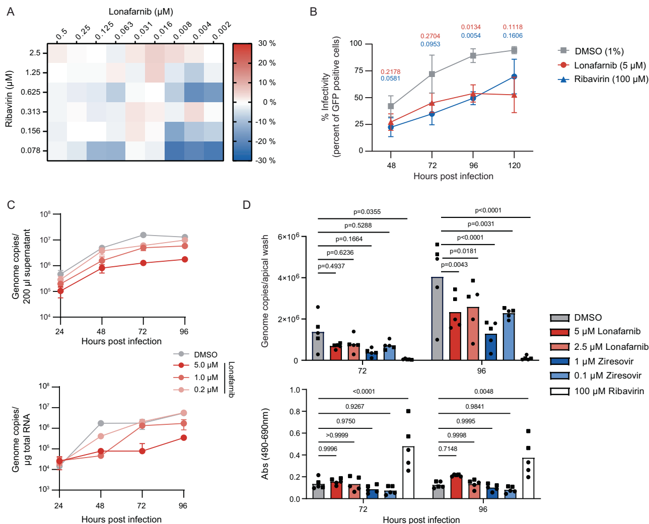
Fig. 7 | Lonafarnib inhibits RSV infection in differentiated human lung cells.
