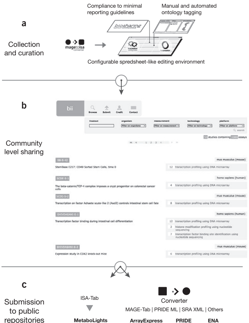
Figure 1 The ISA framework in action in the stem cell–based system of the Harvard Stem Cell Institute (HSCI). The data management workflow of the HSCI’s Stem Cell Discovery Engine (SCDE) system, powered by the ISA framework. (a) Curators use the ISAconfigurator and ISAcreator software modules to consistently curate a variety of internally generated stem cell-based genomics profiles according to community-developed minimum information guidelines and terminologies; published transcriptomics-based studies are also collected via the MAGeToISA module, then curated and enriched for consistency. (b) Consistently represented investigations are loaded in the BioInvestigation Index (BII) component that stores and serves the (public and private) data sets to the HSCI and wider community. (c) Upon publication, investigations are directly submitted to those public repositories using ISA-Tab format, or converted to/from other supported formats via the ISAconverter.
